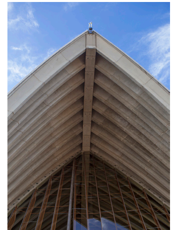
Opera House Concrete Ribbing
