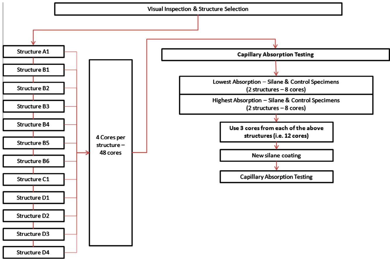
Fig. 4. Selection and testing programme for silane treated cross-beams.
