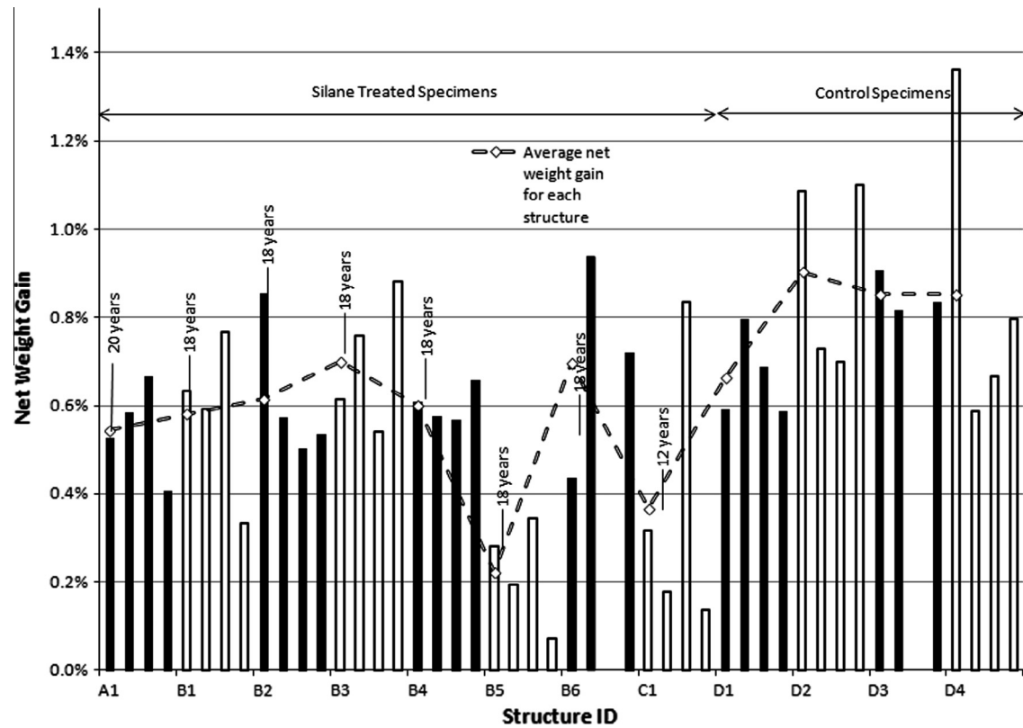
Fig. 7. Net weight gain for each specimen and average net weight gain for each cross-beam's group of specimens after 4 h of capillary absorption testing. Note: The change in color within the vertical bars simply differentiates specimens between different cross-beams. The age of the silane at time of testing is also noted.
