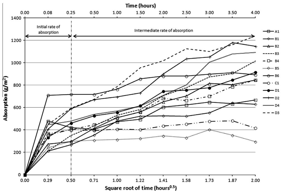
Fig. 8. Average cumulative absorption for each cross-beam's group of specimens over 4 h of capillary absorption testing.
