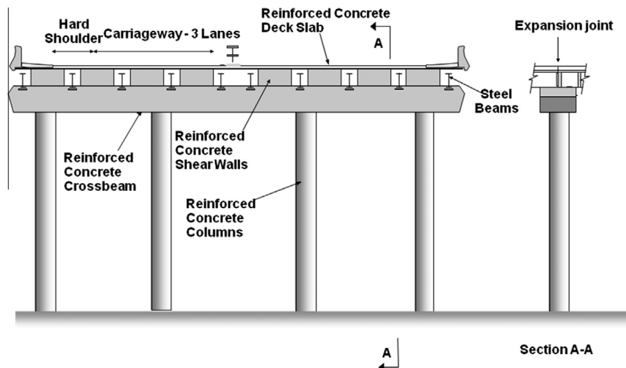
Fig. 3. Typical sub-structure arrangement of the UK's Midland Links Motorway Viaducts (MLMV).
