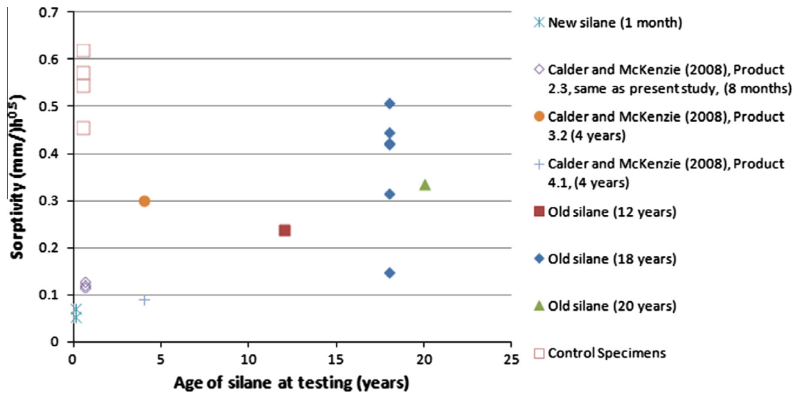
Fig. 9. Comparison of the sorptivity of silane treated specimens examined in the study against the sorptivity of specimens from Calder and McKenzie [22].
